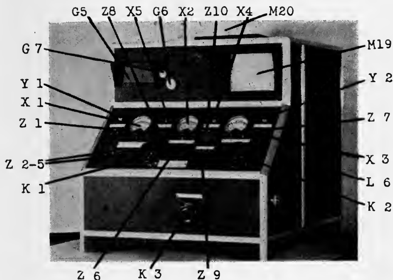
FIG. 4. Photograph of graininess photometer fully assembled.
